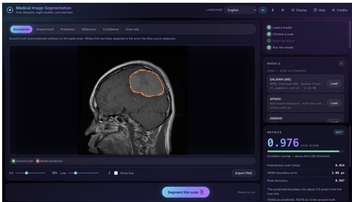
Figure 12 ADIT, Task 2. Her EfficientNet-B4 encoder U-Net on report case 627, Dice 0.976 from the recorded results
