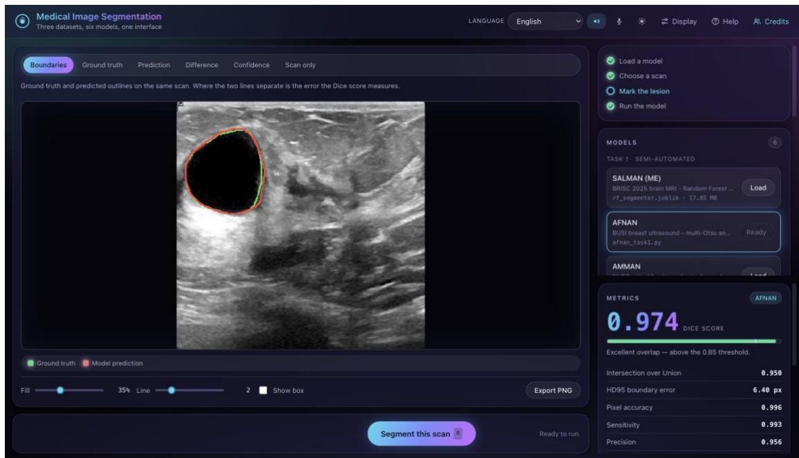
Figure 7 AFNAN, Task 1. The classical pipeline on a benign BUSI lesion, Dice 0.974. The box controls are gone because this method finds the lesion itself
